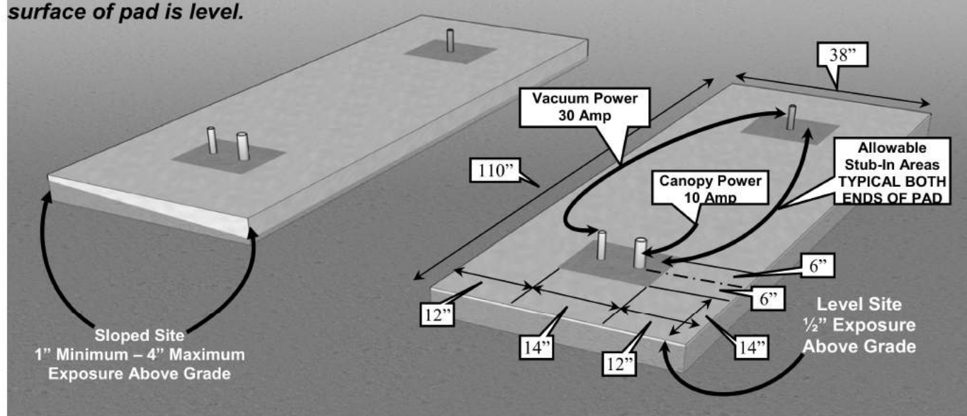
Figure 1 – Concrete Pad 6" Thick
